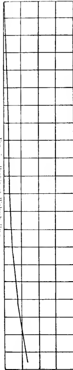
FIG. 5. Profile of Welsh River.
